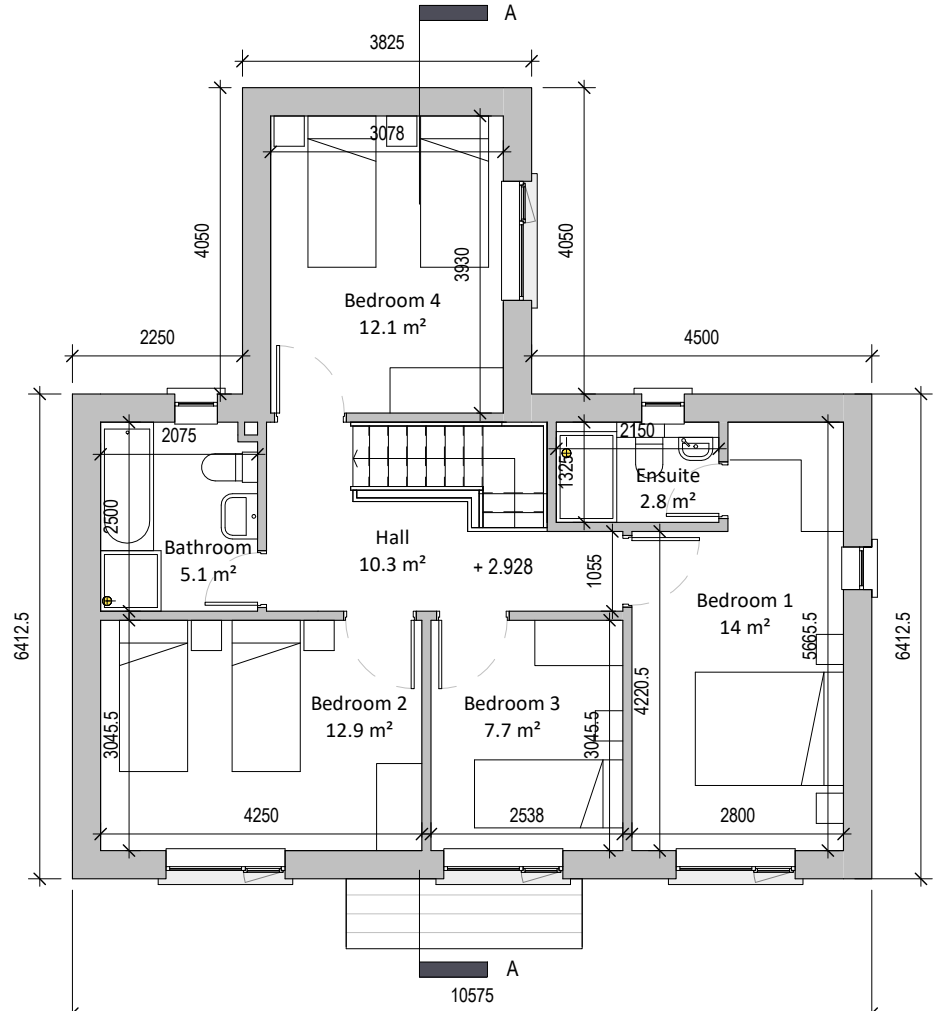
2 First Floor 1 : 100
