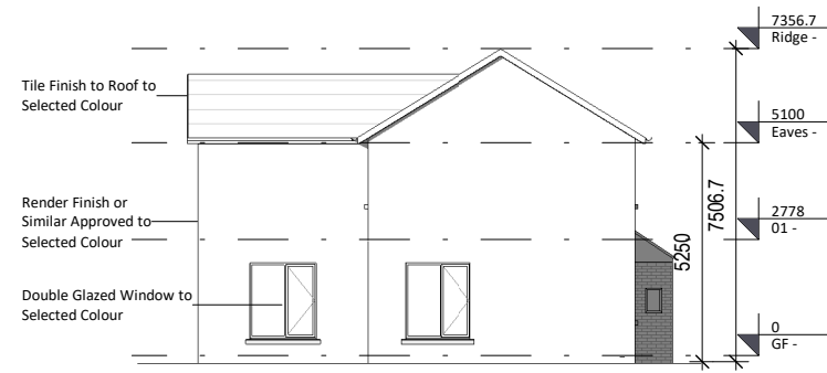
6 Gable Elevation 02 1 : 200
