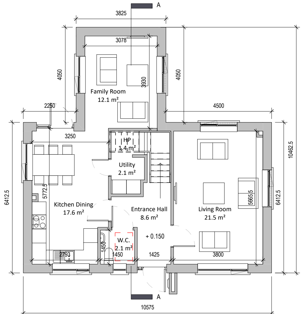
1 Ground Floor 1 : 100
